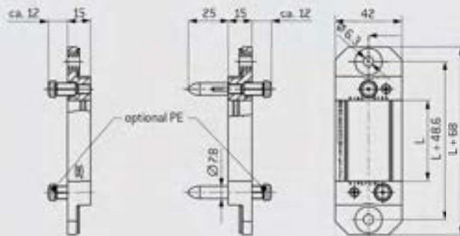
PIN FRAME WITH GUIDING PIN
