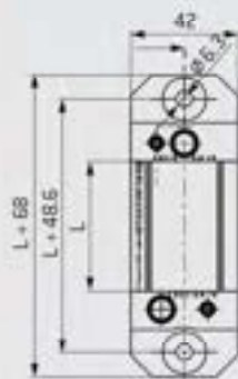
SOCKET FRAME WITH GUIDING BUSHES
