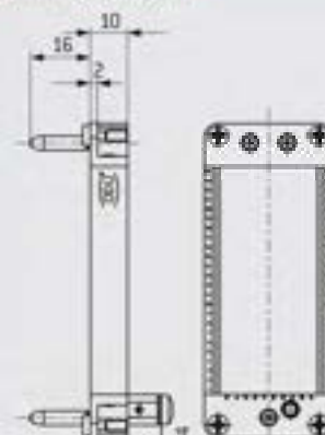
PIN FRAME WITH GUIDING PIN
