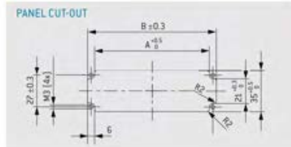
DIRECT ASSEMBLY OF THE SOCKET FRAME ON ASSEMBLY WALL
