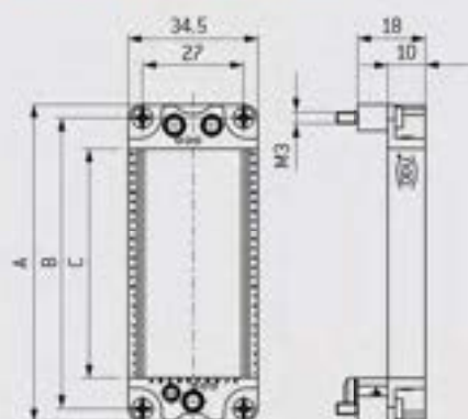
SOCKET FRAME WITH GUIDING BUSHES
