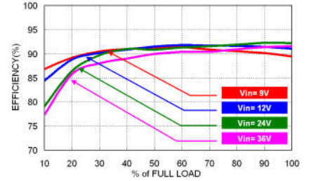
RED40-24S05W Efficiency vs. Output Load
