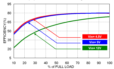
MPS(H)02-05S05 Efficiency vs. Output Current
