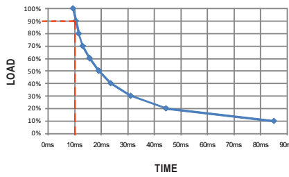
RSD-300E-48
