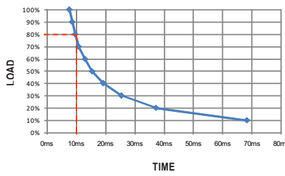
RSD-300E-48
