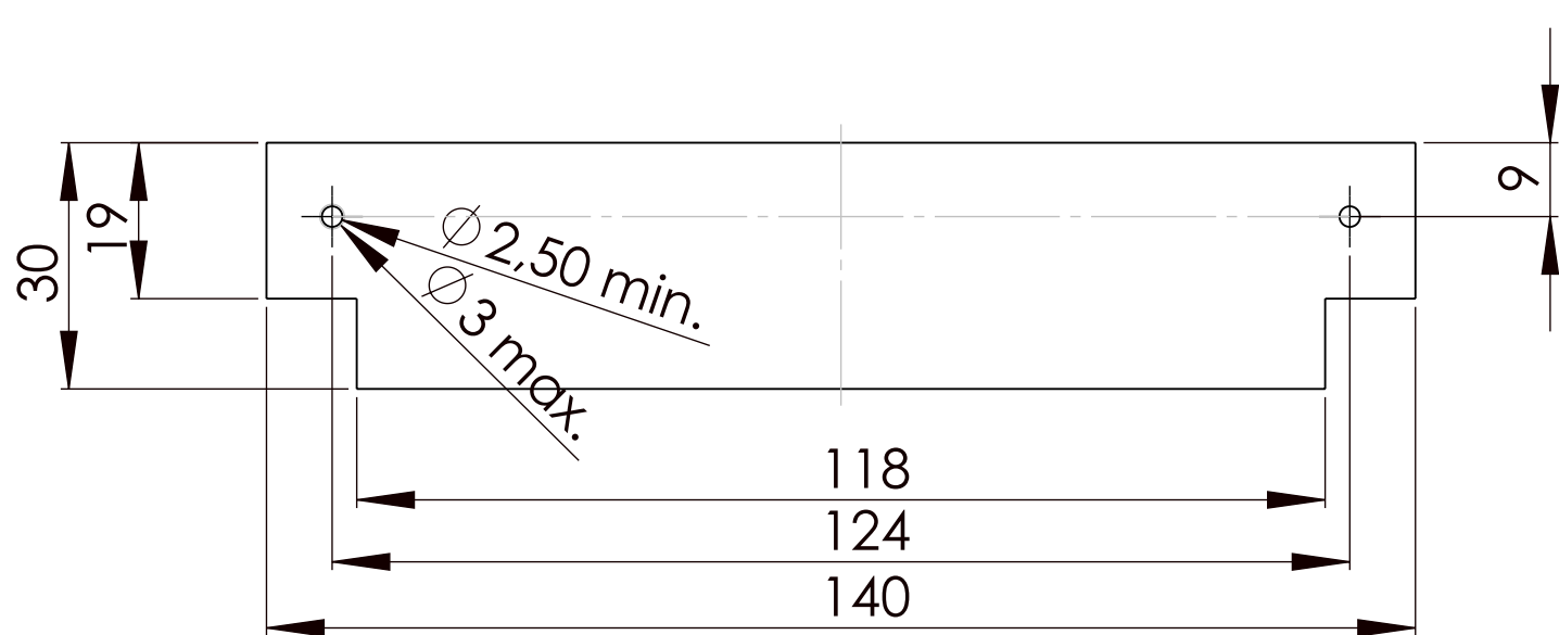
Platine UT Batteriefach P C B battery-compartment
