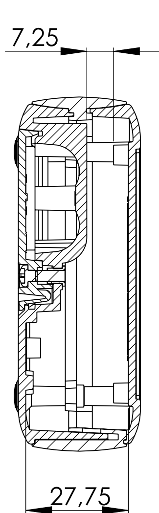
B-B with battery compartment
