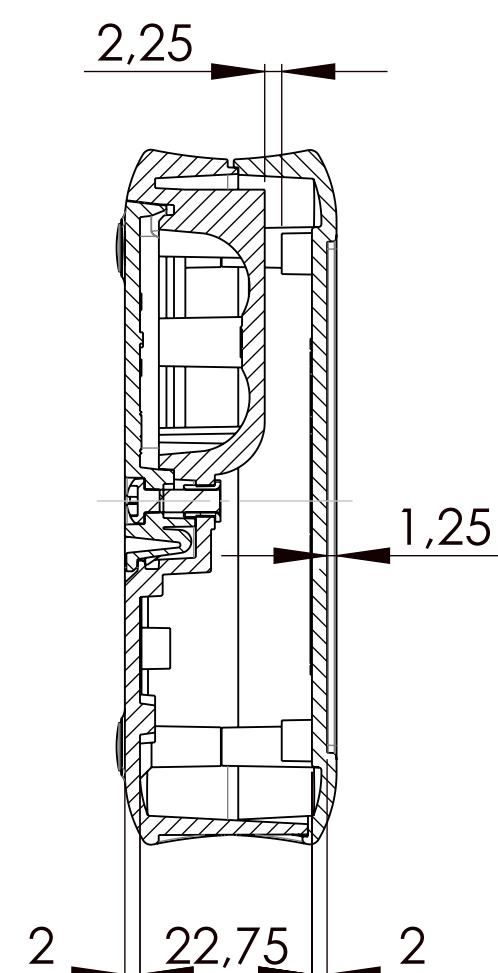
A-A with battery component
