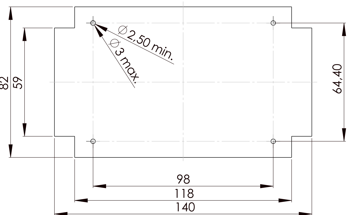
Platine OT P C B
