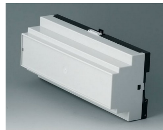
B6506113 RAILTEC B, 12 modules, Vers. III PC (UL 94 V-0) light grey RAL 7035 210x90x58mm
