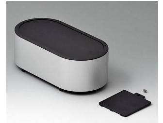
EO206059 SYNERGY O200 Aluminium AlMgSi 0.5 matt anodised 200x100x70mm IP 40
